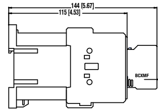
Vdc Contactors
