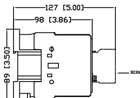
Vac Contactors
