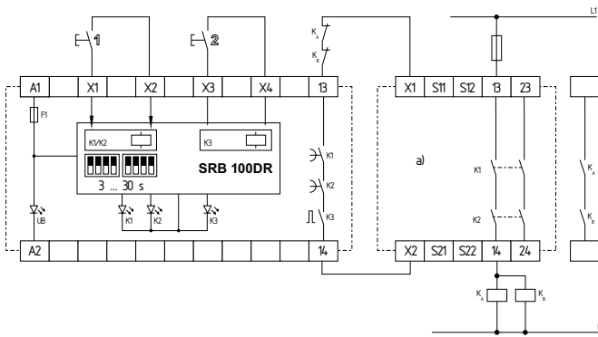
Fig. 3 a) SRB, eg. SRB 301ST or SRB 211ST
