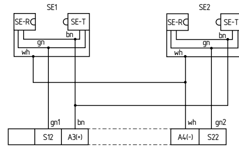
Connection of 2 safety edges (signal generators)
