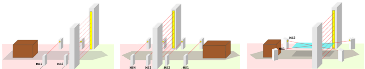
2 sensors - 1 directional muting MUT-SET-L-01, MUT-SET-L-02
