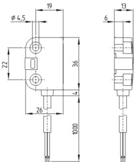
Dimensional drawing (basic component)
