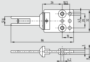
Straight actuator EX-BO
