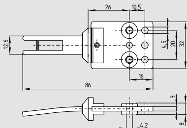
Straight radius actuator EX-BOR
