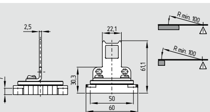
Angled actuator B5-Flex
