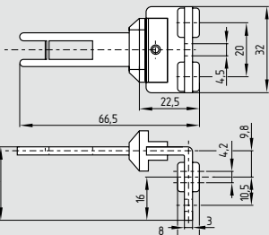
Angled actuator EX-BOW
