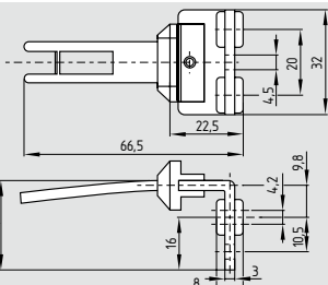
Angled radius actuator EX-BOWR
