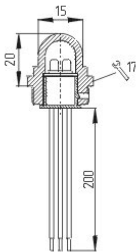
Dimensional drawing (basic component)
