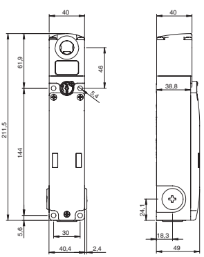
Switch NG 2D6D••1A Operating principle D, with key release and escape release button, without actuator
