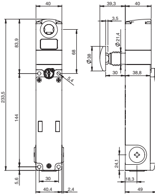
Switch NG 2D7D••1A Operating principle D, with escape release button, without actuator
