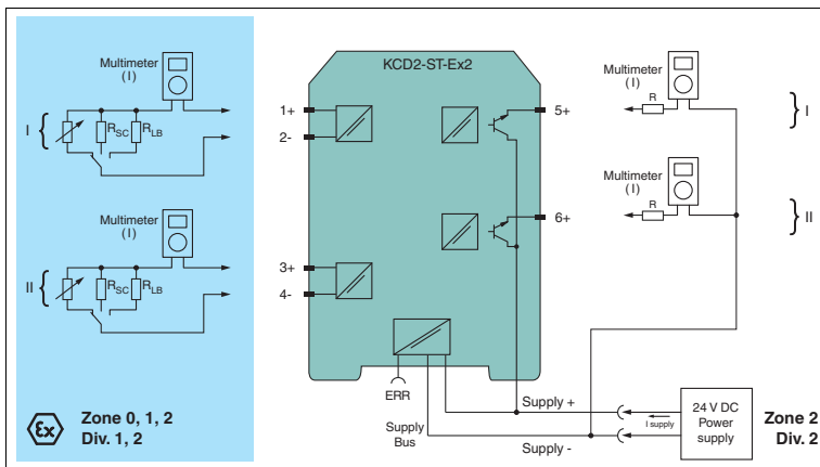
Figure 4.2 Proof test set-up for KCD2-ST-(Ex)2(.SP)
