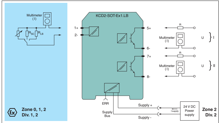
Figure 4.3 Proof test set-up for KCD2-SOT-(Ex)1.LB.(SP)
