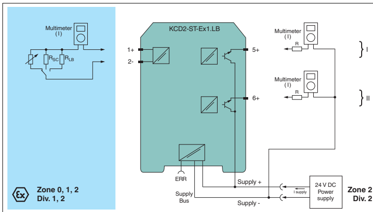
Figure 4.1 Proof test set-up for KCD2-ST-(Ex)1.LB(.SP)
