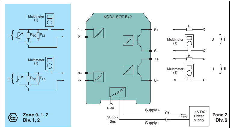
Figure 4.4 Proof test set-up for KCD2-SOT-(Ex)2.(SP)
