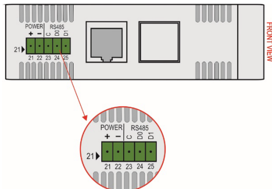
Figure 11 – RS485 connection
