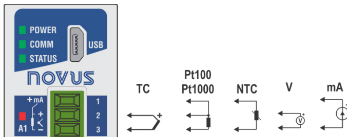
Figure 14 – TC / Pt100 / Pt1000 / NTC / V / mA
