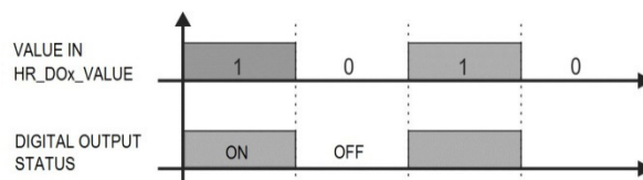
Figure 20 – "Logical Status" mode
