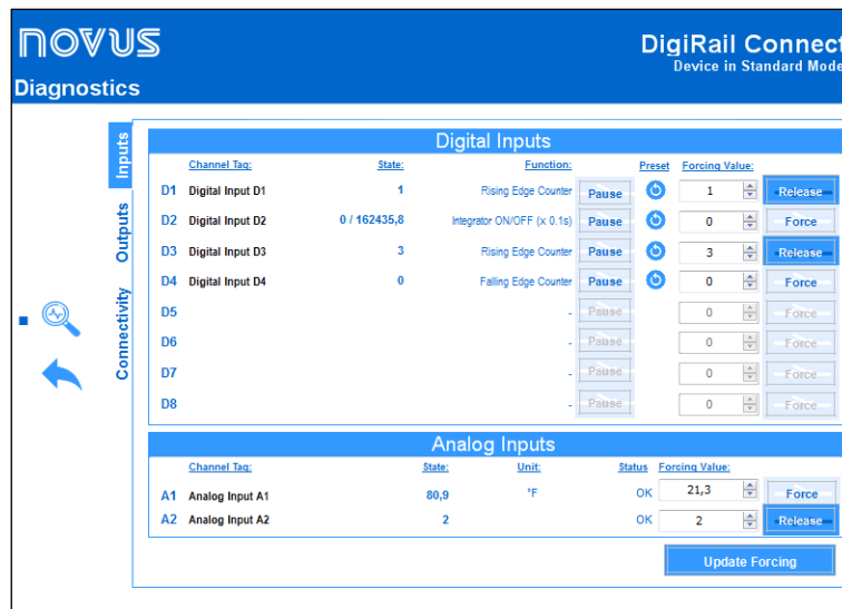
Figure 33 – Diagnostics: Inputs
