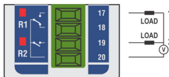
Figure 25 – Relay
