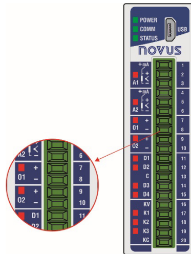
Figure 17 – Analog Outputs
