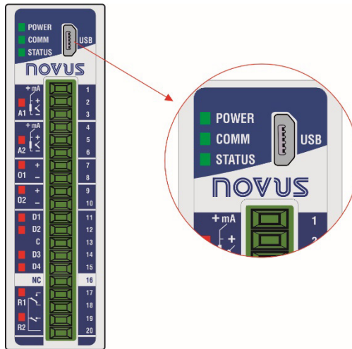
Figure 10 – USB connection
