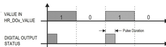
Figure 21 – "Pulse" mode
