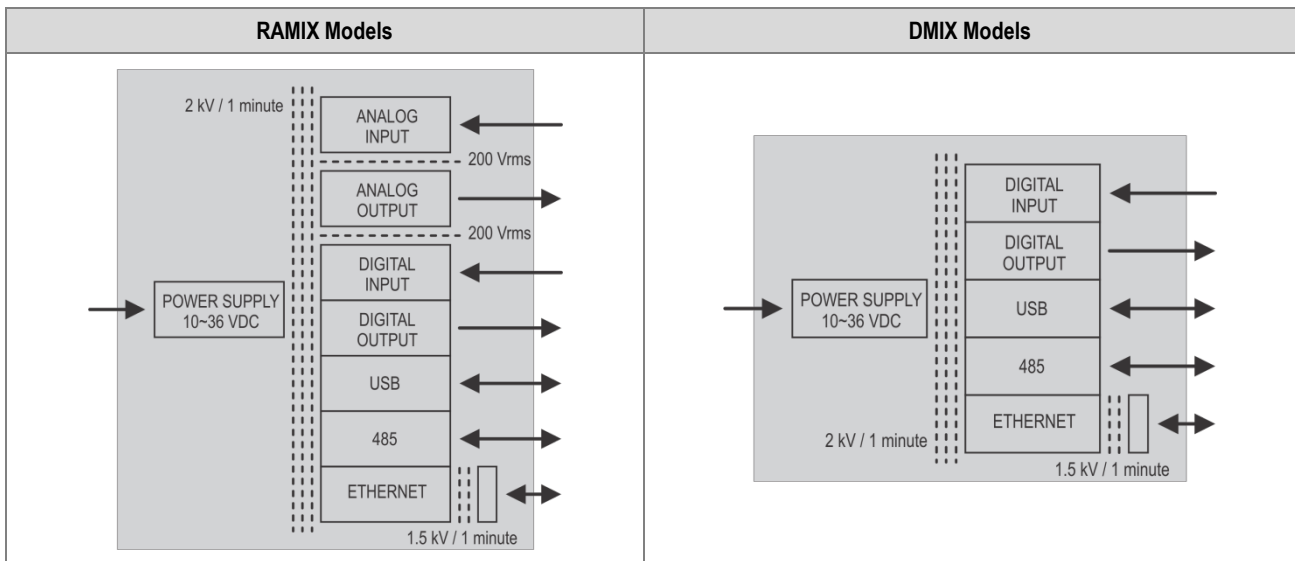
Figure 12 – Galvanic isolation
