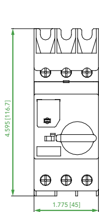
Ex9S32 + CCE51 Unit: in [mm]
