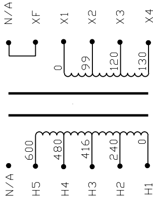
CONNECTION DIAGRAM
