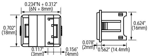
Enplate (DL9Z - 5W - _)
