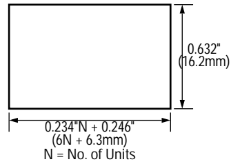
Panel Cut-Out (when using end plate Part No. DL9Z-5W)
