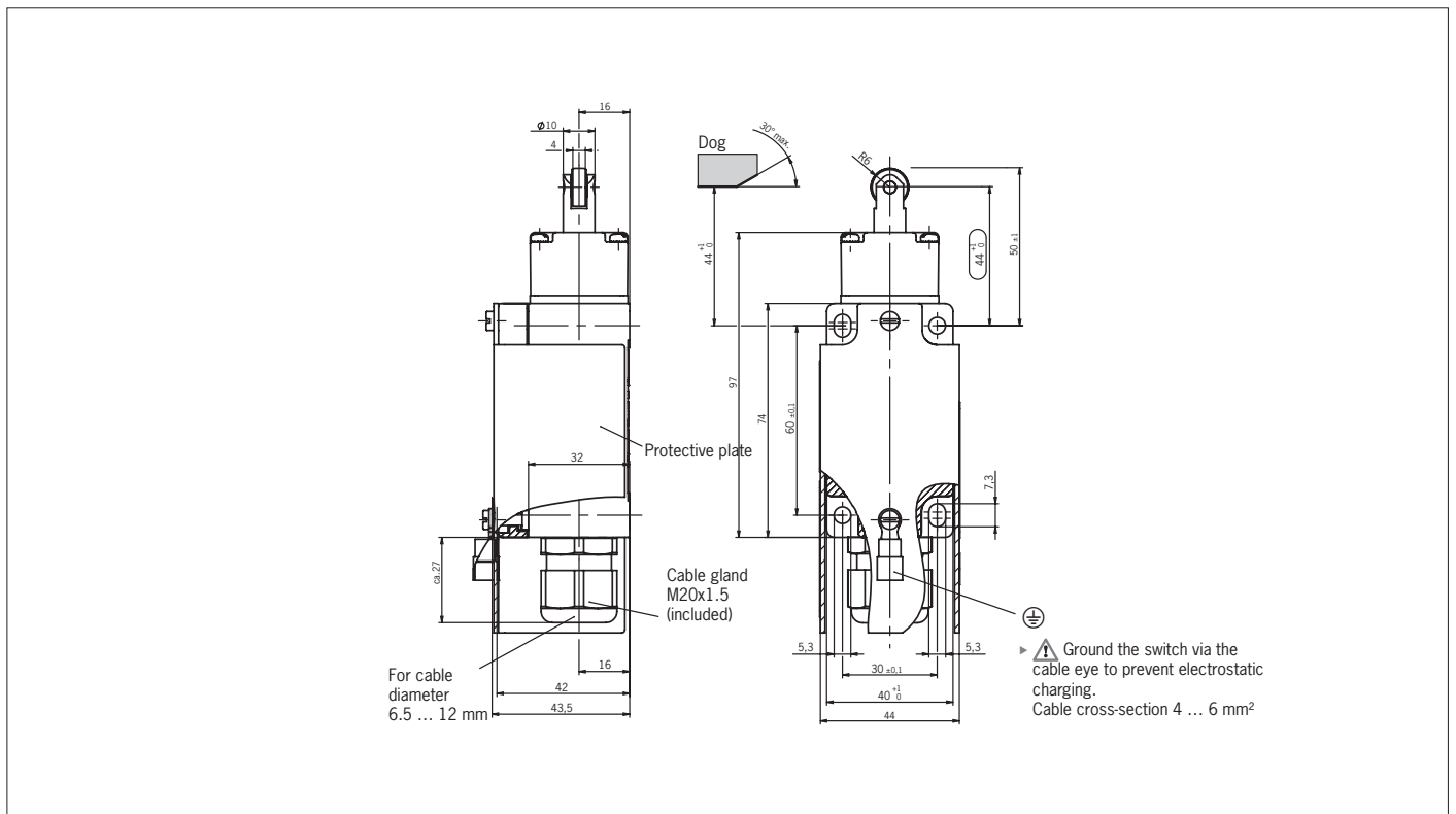
Fig. 4: Dimension drawing for NZ1...EX
