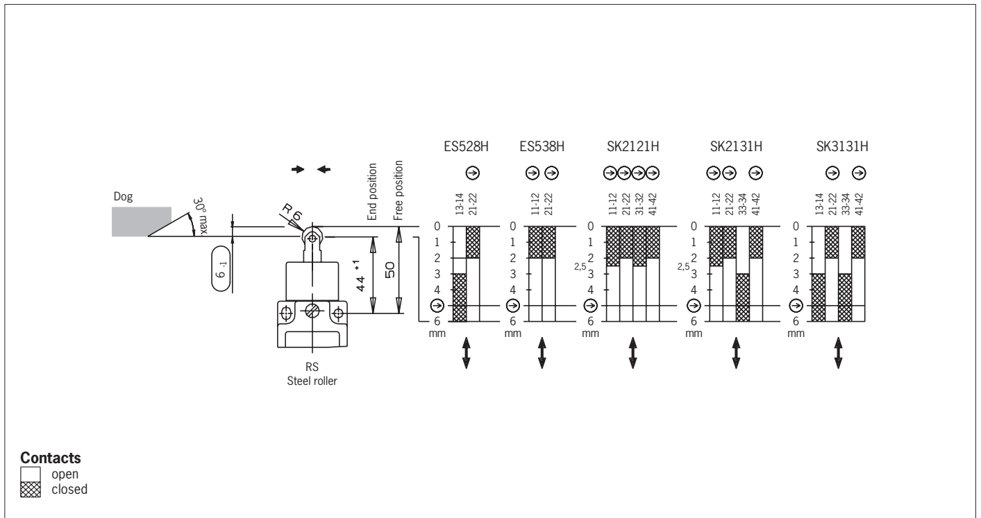
Fig. 2: Travel diagrams, actuator and approach directions
