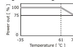
Fig. 5 Derating
