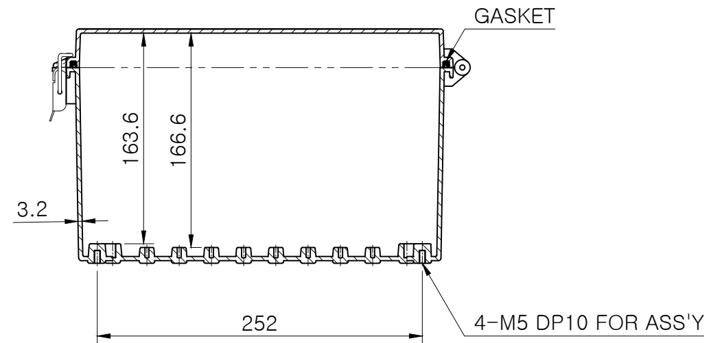
SECTION B-B
