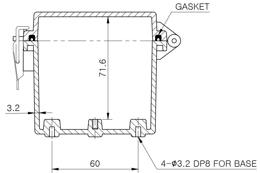
SECTION B-B
