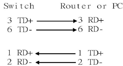
Straight Through Cable Schematic
