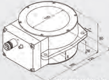
KJR-D100AN-DNA-V2 KJR-D100AN-DPA-V2
